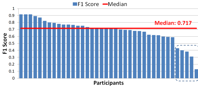
Figure 3. F1 score between self-report and sensor assessment range from 0.130 to 0.917 with median 0.717. Bottom 5 have unacceptable self-report consistency score with median cronbach’s alpha score 0.335 while overall consistency score is 0.843.
