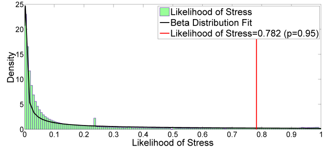
Figure 5. The likelihood of stress follow beta distribution with shape parameter \alpha = 0.222 and \beta = 1.027 . Significant stress threshold is 0.782 ( p=0.95 ).
