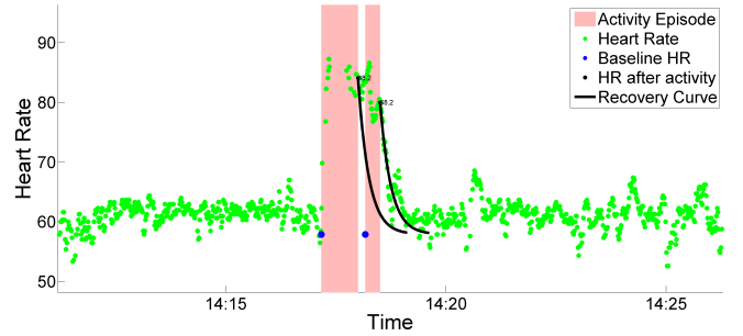
Figure 2. Heart-rate increases due to activity. Exponential recovery parameter \tau is learnt for each participant. 99% exponential recovery curve (equation 1) is shown. Before the heart rate is recovered another activity happened. So baseline heart rate is carry forwarded.
