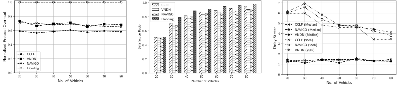
Figure 8: Performance of CCLF, VNDN, Navigo, and Flooding with Geo-location Information
